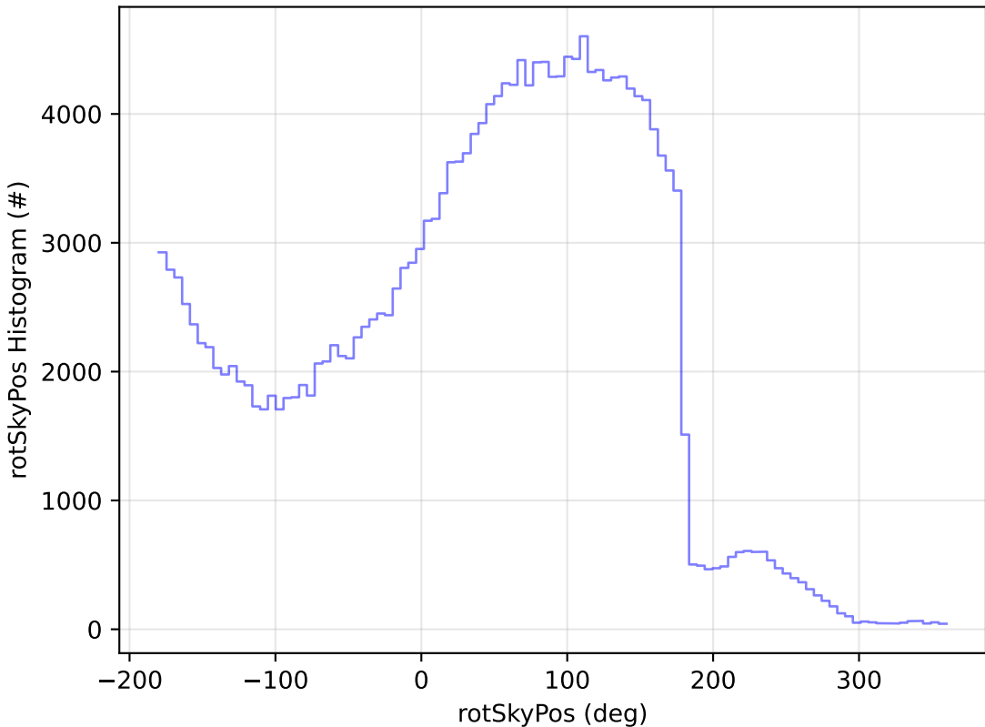
telescope_jerk_v3.5_10yrs All sky g band: rotSkyPos Histogram
