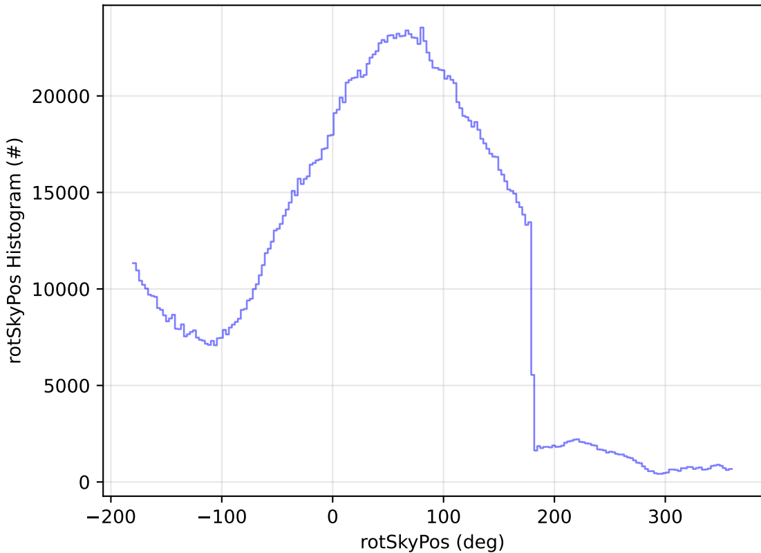
telescope_jerk_v3.5_10yrs All sky all bands: rotSkyPos Histogram
