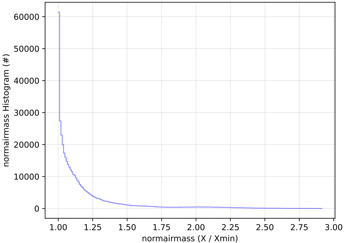
telescope_jerk_v3.5_10yrs WFD z band: normairmass Histogram
