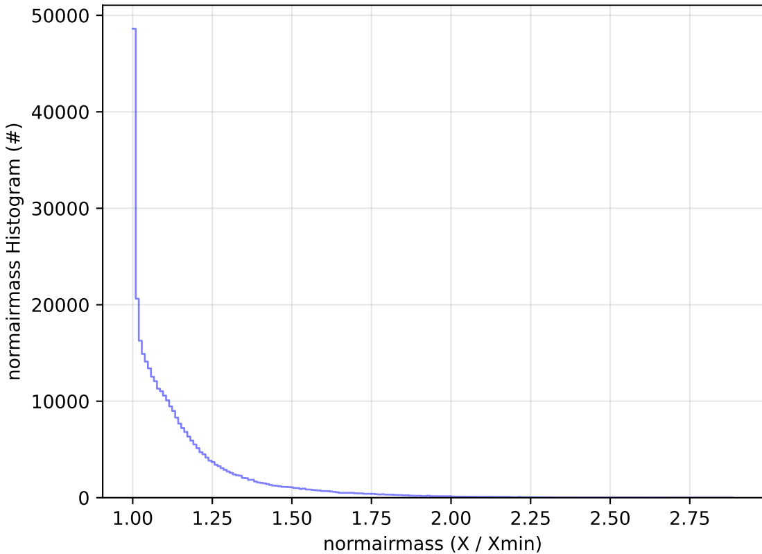
telescope_jerk_v3.5_10yrs WFD y band: normairmass Histogram
