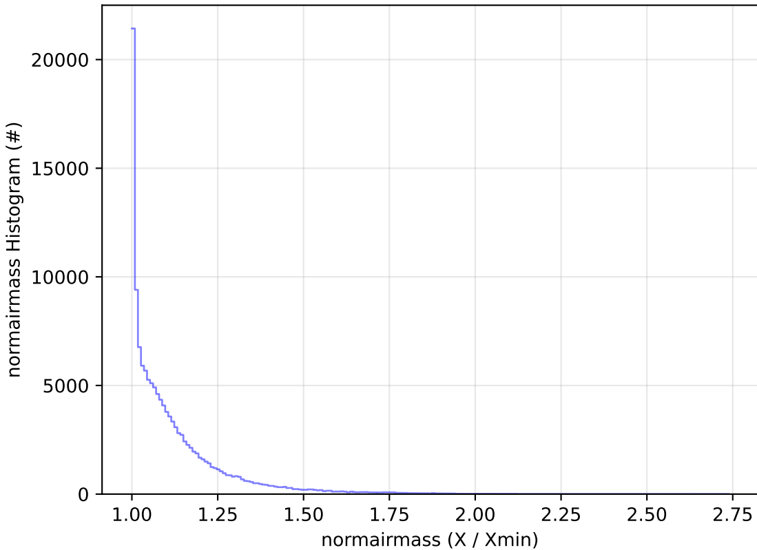
telescope_jerk_v3.5_10yrs WFD u band: normairmass Histogram
