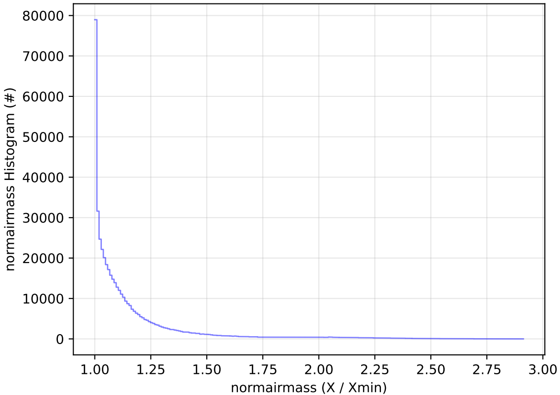
telescope_jerk_v3.5_10yrs WFD r band: normairmass Histogram
