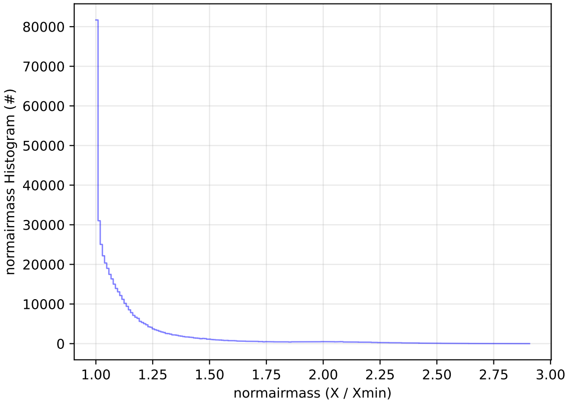
telescope_jerk_v3.5_10yrs WFD i band: normairmass Histogram
