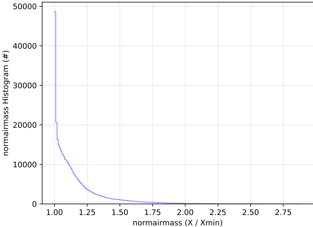
telescope_jerk_v3.5_10yrs All sky y band: normairmass Histogram
