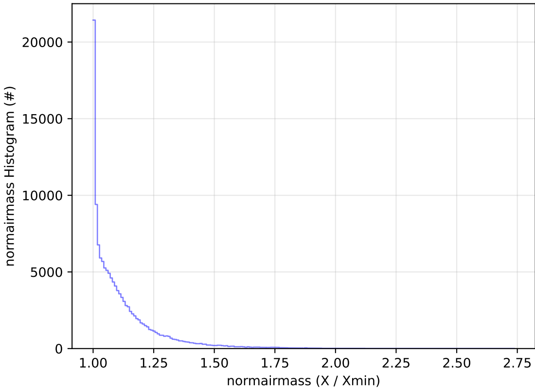
telescope_jerk_v3.5_10yrs All sky u band: normairmass Histogram
