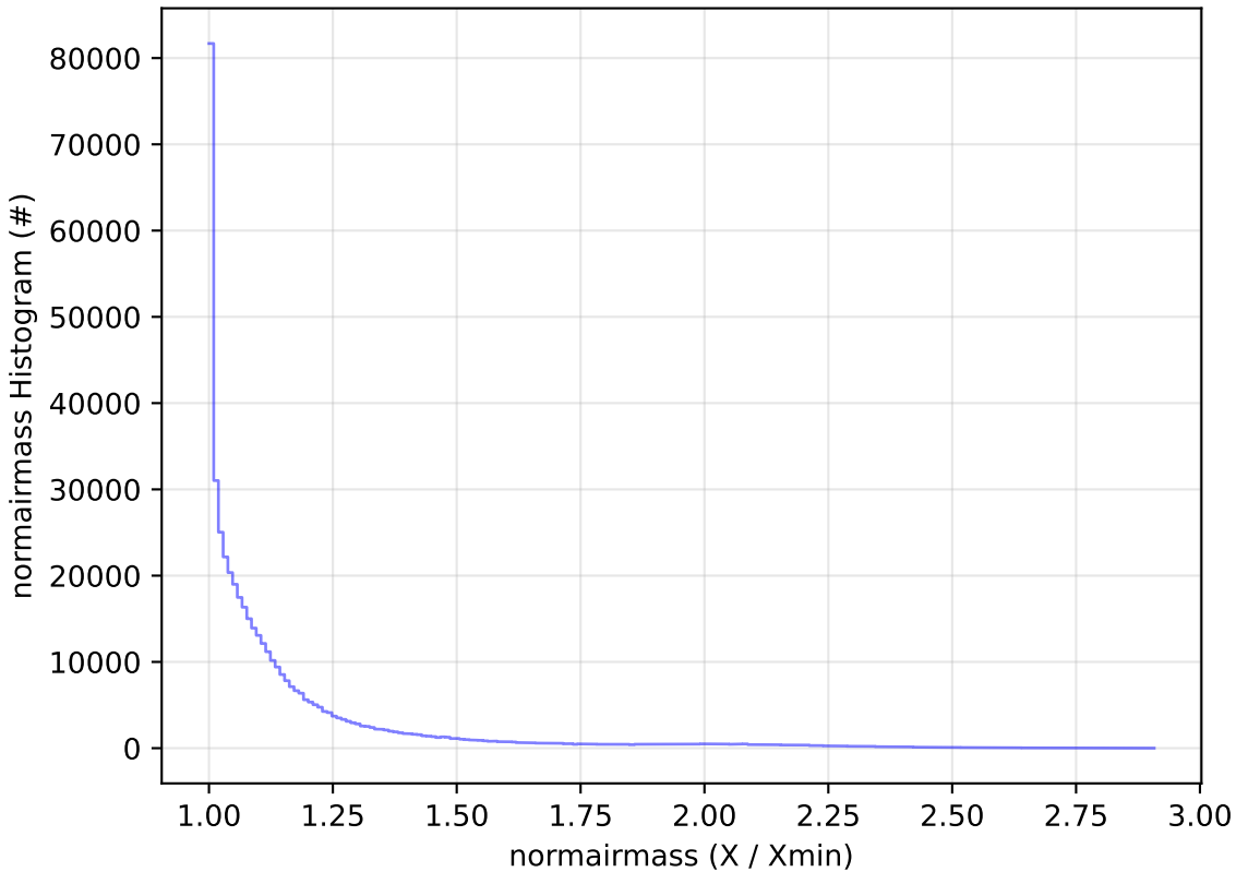
telescope_jerk_v3.5_10yrs All sky i band: normairmass Histogram
