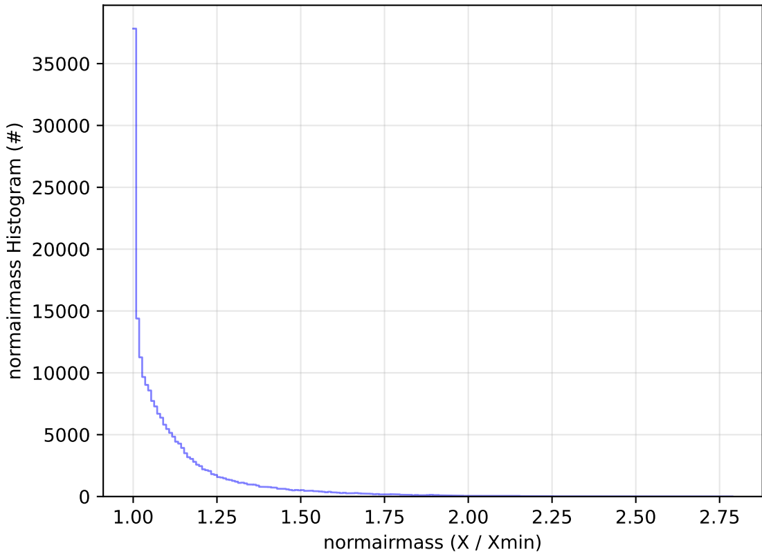
telescope_jerk_v3.5_10yrs All sky g band: normairmass Histogram
