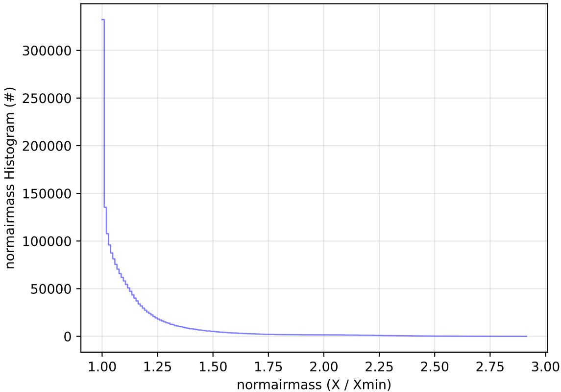
telescope_jerk_v3.5_10yrs All sky all bands: normairmass Histogram
