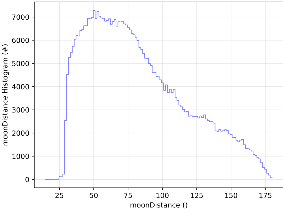
telescope_jerk_v3.5_10yrs WFD z band: moonDistance Histogram
