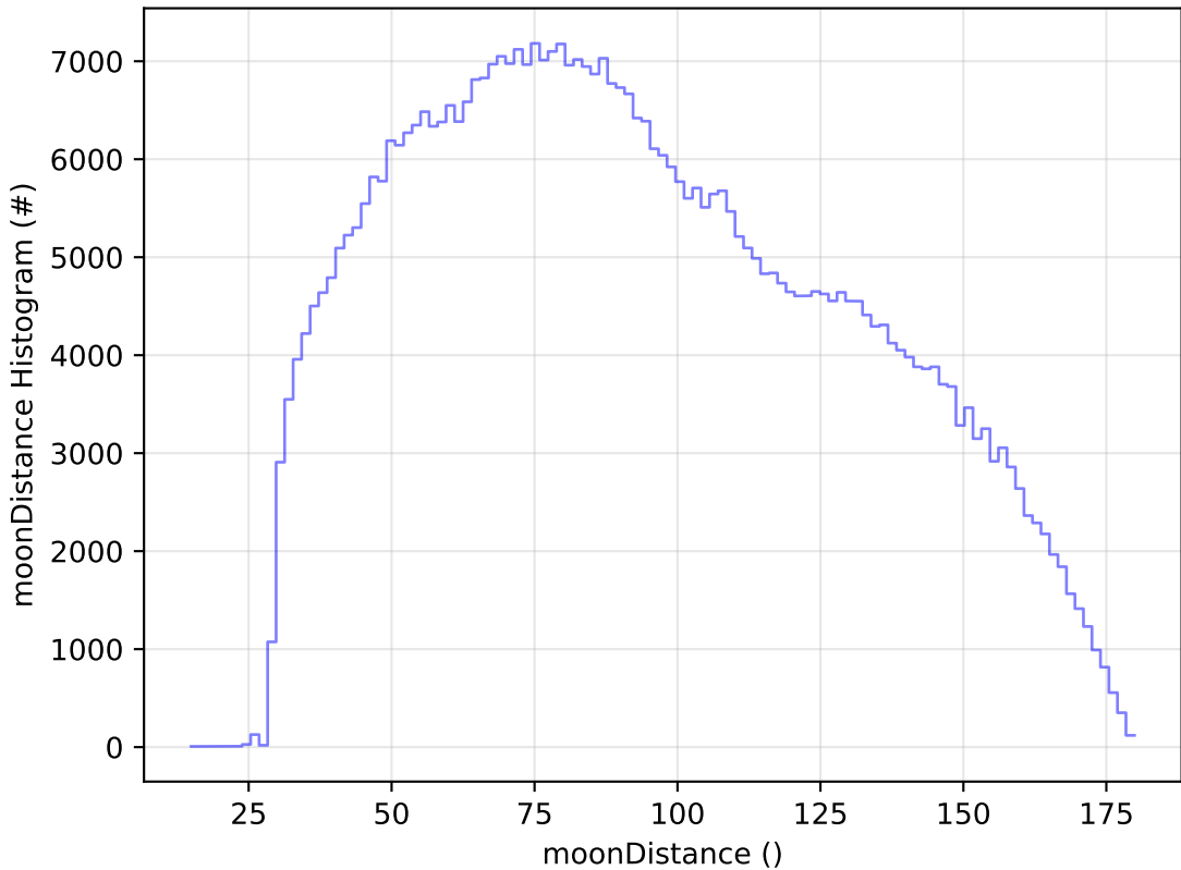
telescope_jerk_v3.5_10yrs WFD i band: moonDistance Histogram
