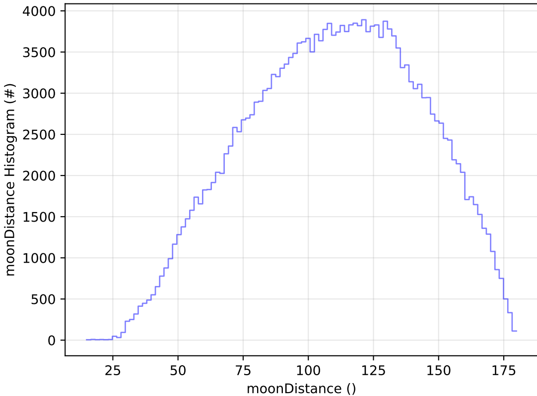
telescope_jerk_v3.5_10yrs WFD g band: moonDistance Histogram
