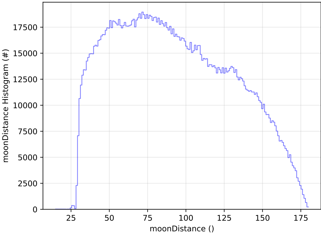
telescope_jerk_v3.5_10yrs WFD all bands: moonDistance Histogram
