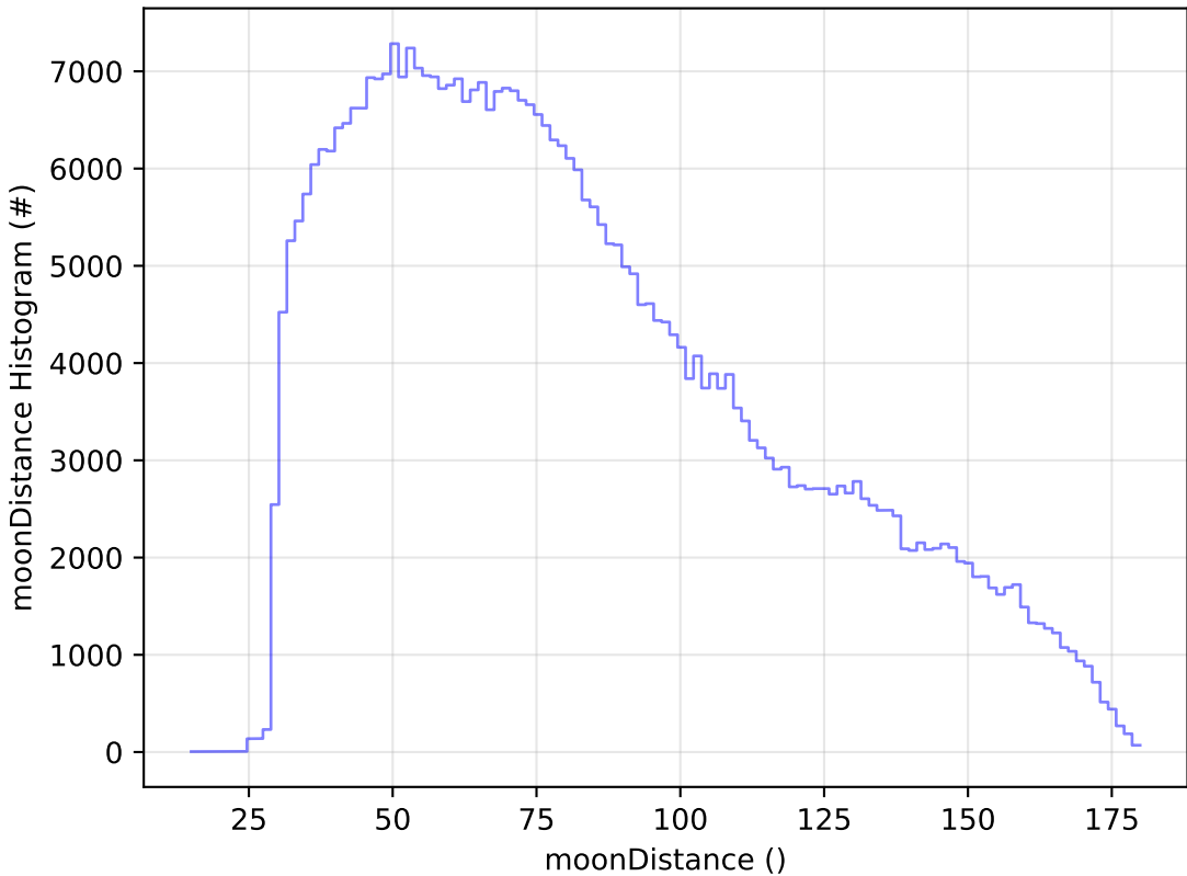
telescope_jerk_v3.5_10yrs All sky z band: moonDistance Histogram
