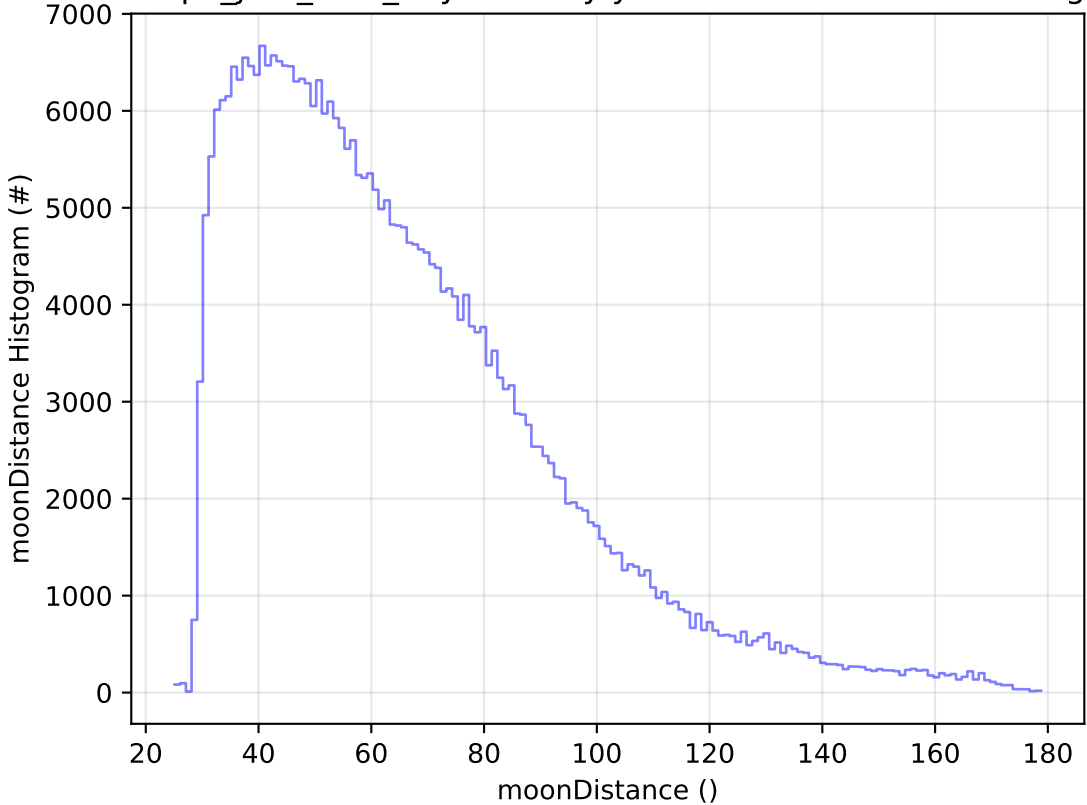
telescope_jerk_v3.5_10yrs All sky y band: moonDistance Histogram
