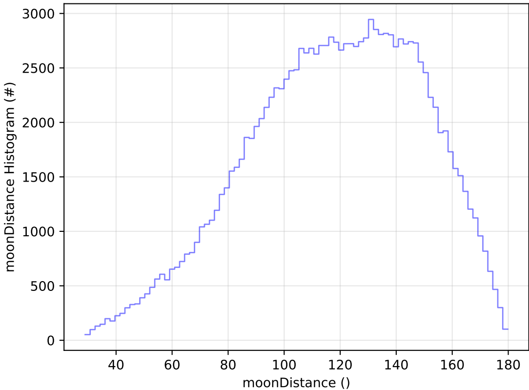
telescope_jerk_v3.5_10yrs All sky u band: moonDistance Histogram
