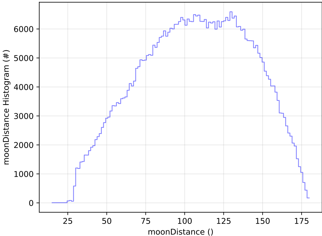
telescope_jerk_v3.5_10yrs All sky r band: moonDistance Histogram
