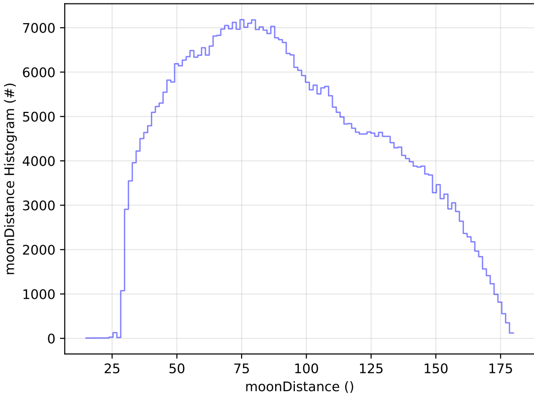
telescope_jerk_v3.5_10yrs All sky i band: moonDistance Histogram
