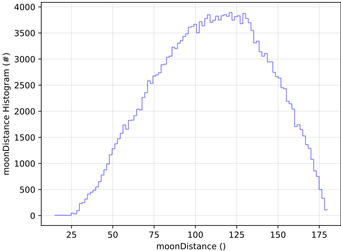
telescope_jerk_v3.5_10yrs All sky g band: moonDistance Histogram
