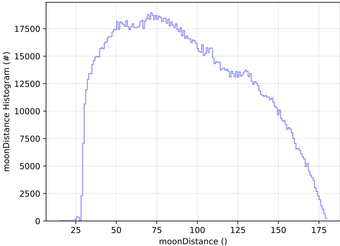
telescope_jerk_v3.5_10yrs All sky all bands: moonDistance Histogram
