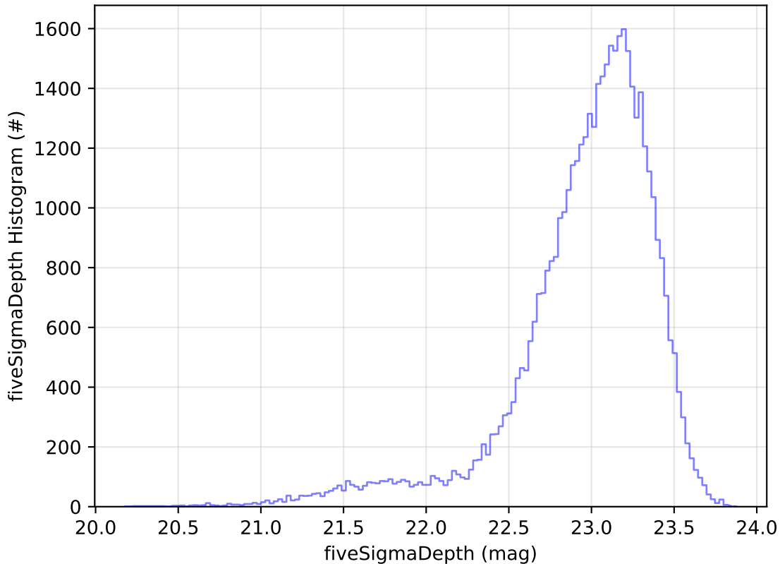
telescope_jerk_v3.5_10yrs Yr 1 z band: fiveSigmaDepth Histogram
