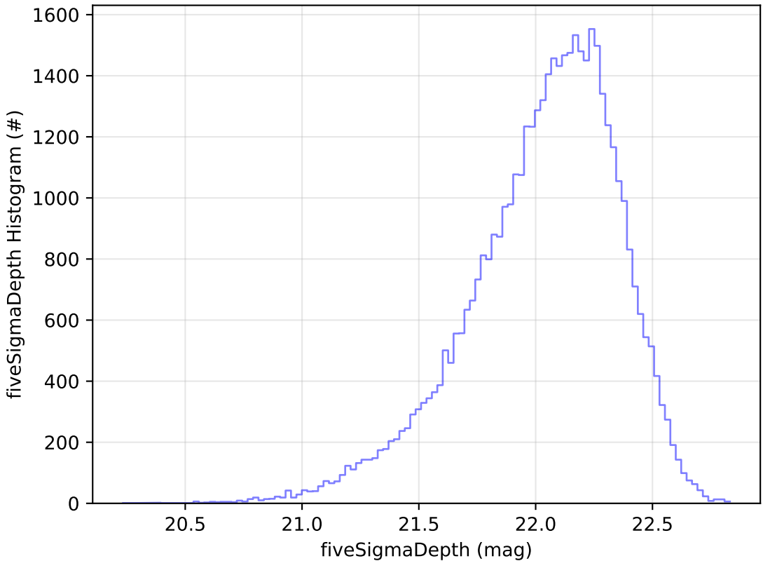
telescope_jerk_v3.5_10yrs Yr 1 y band: fiveSigmaDepth Histogram
