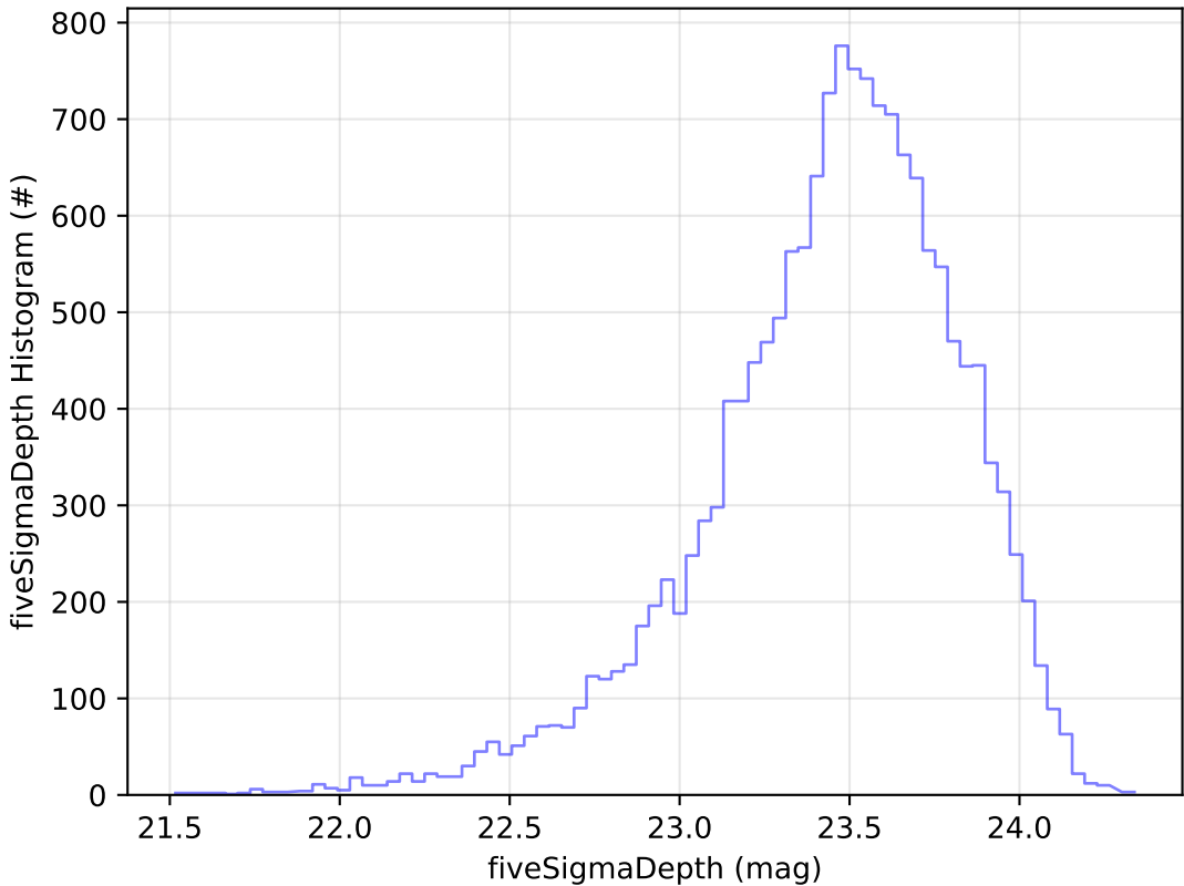
telescope_jerk_v3.5_10yrs Yr 1 u band: fiveSigmaDepth Histogram
