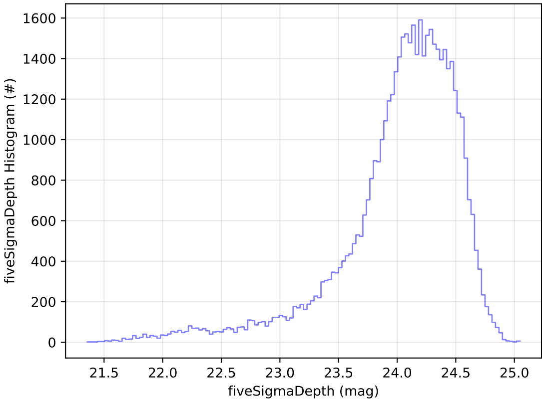
telescope_jerk_v3.5_10yrs Yr 1 r band: fiveSigmaDepth Histogram
