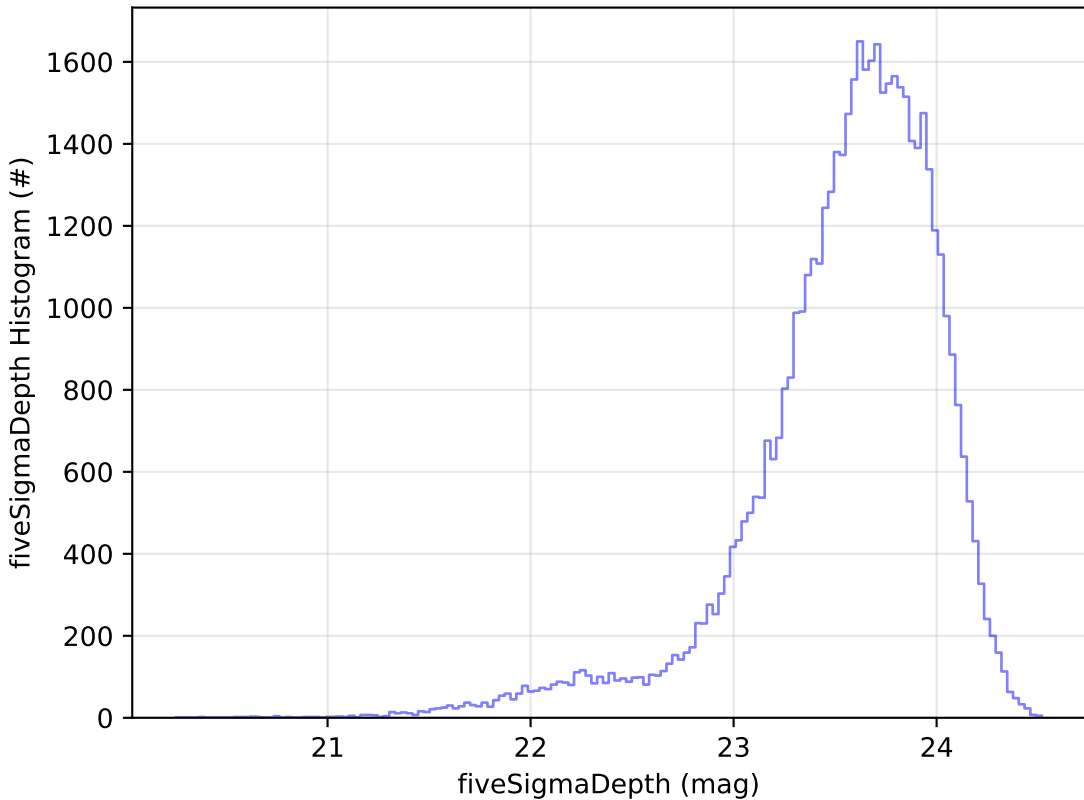
telescope_jerk_v3.5_10yrs Yr 1 i band: fiveSigmaDepth Histogram
