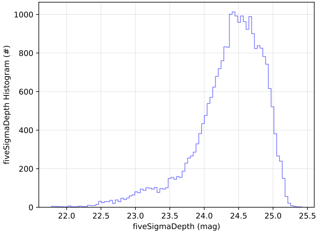
telescope_jerk_v3.5_10yrs Yr 1 g band: fiveSigmaDepth Histogram
