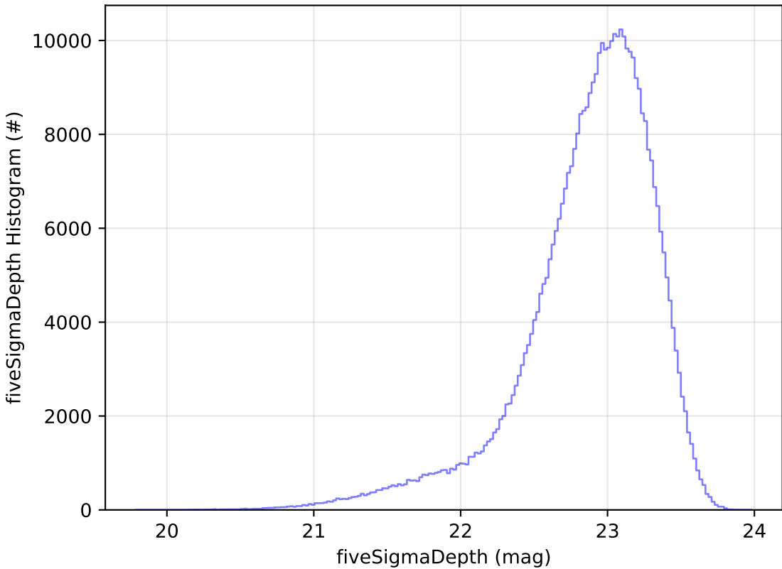
telescope_jerk_v3.5_10yrs WFD z band: fiveSigmaDepth Histogram
