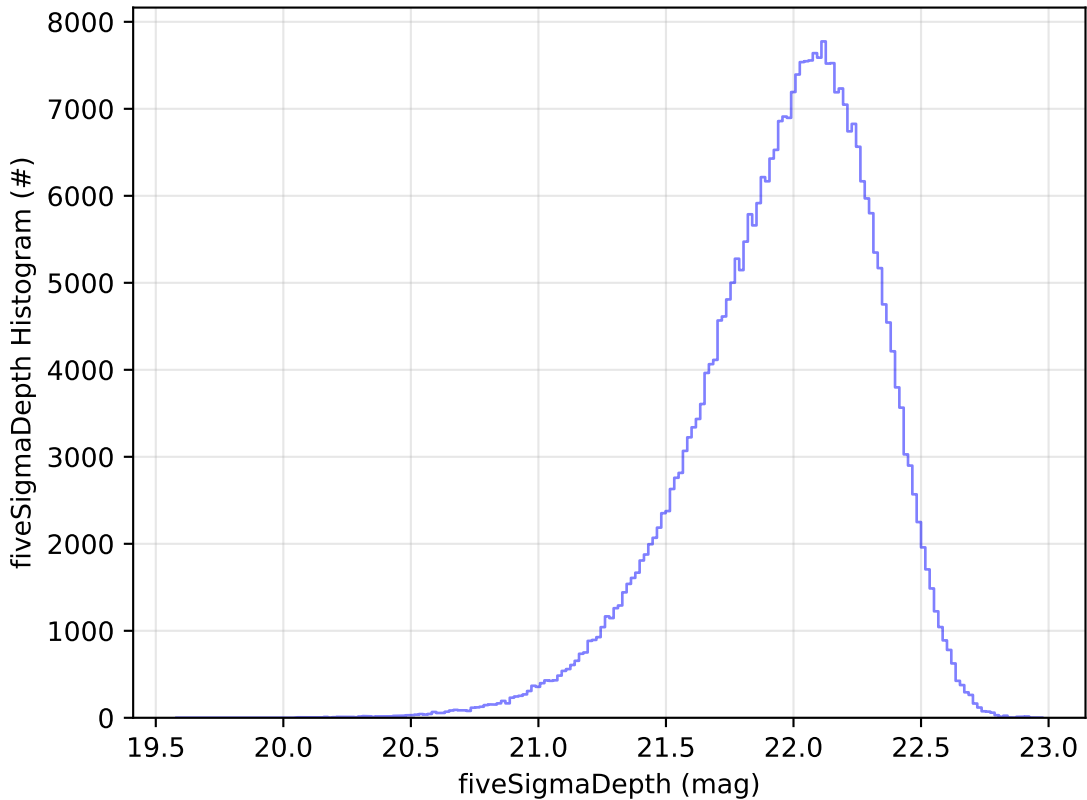
telescope_jerk_v3.5_10yrs WFD y band: fiveSigmaDepth Histogram
