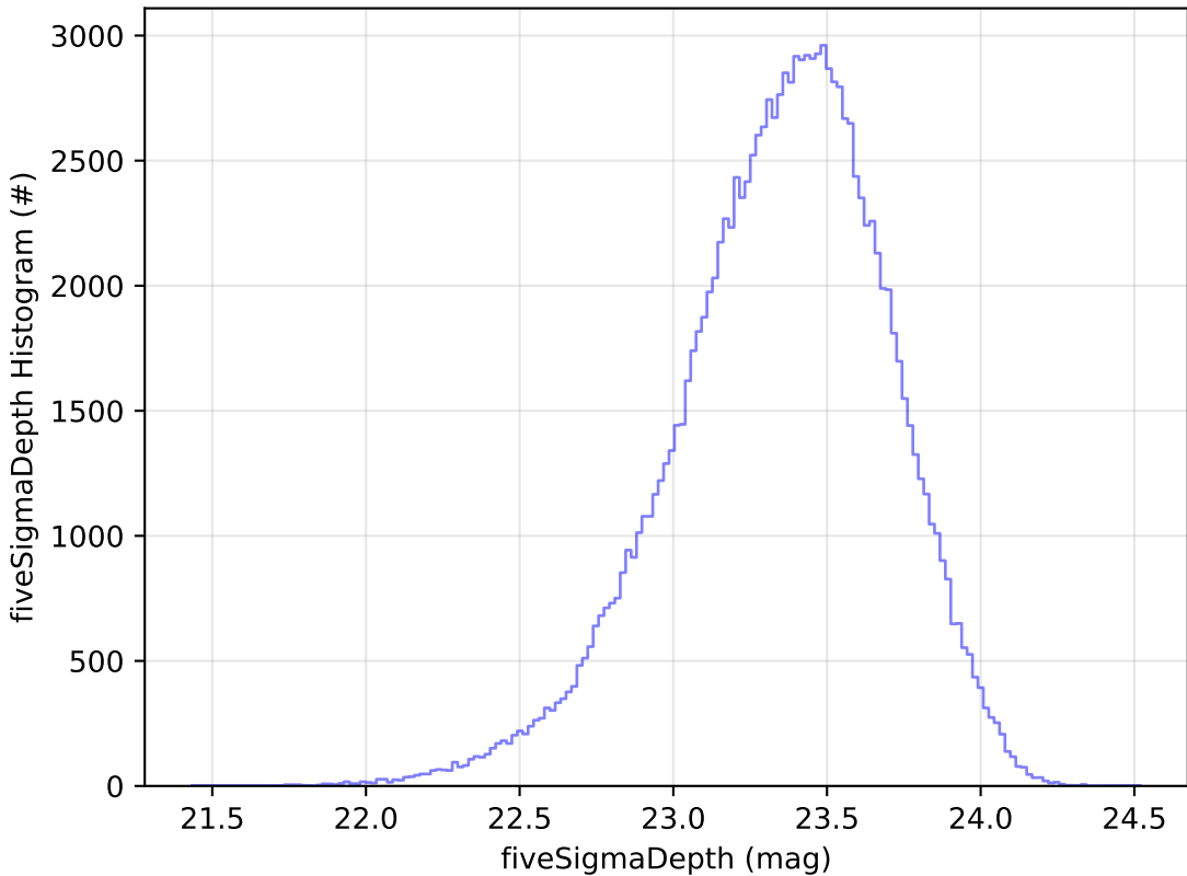
telescope_jerk_v3.5_10yrs WFD u band: fiveSigmaDepth Histogram
