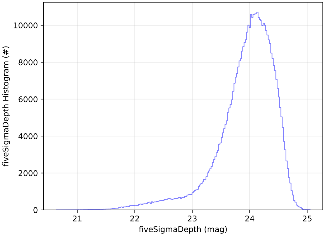
telescope_jerk_v3.5_10yrs WFD r band: fiveSigmaDepth Histogram
