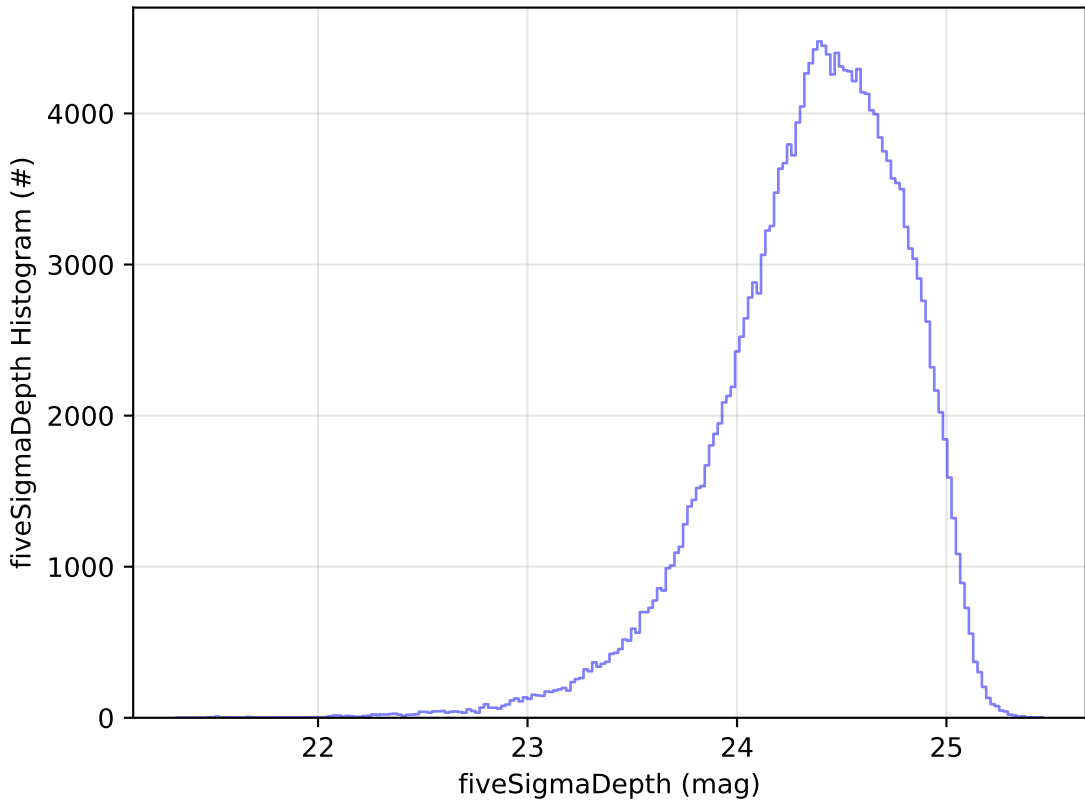
telescope_jerk_v3.5_10yrs WFD g band: fiveSigmaDepth Histogram
