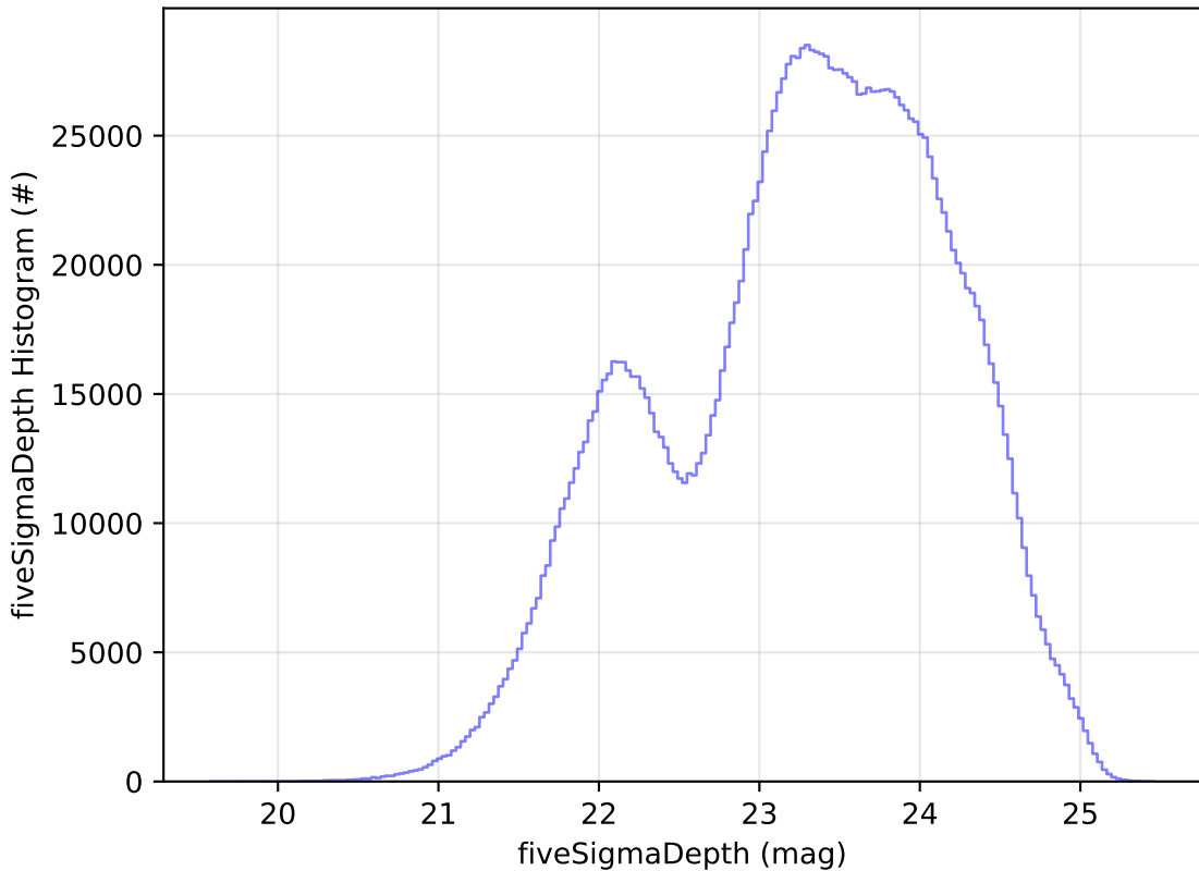
telescope_jerk_v3.5_10yrs WFD all bands: fiveSigmaDepth Histogram
