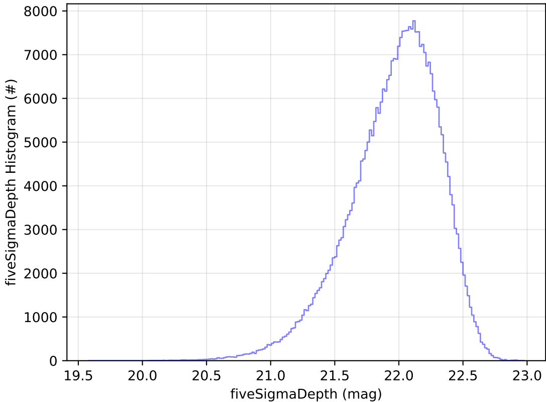
telescope_jerk_v3.5_10yrs All sky y band: fiveSigmaDepth Histogram
