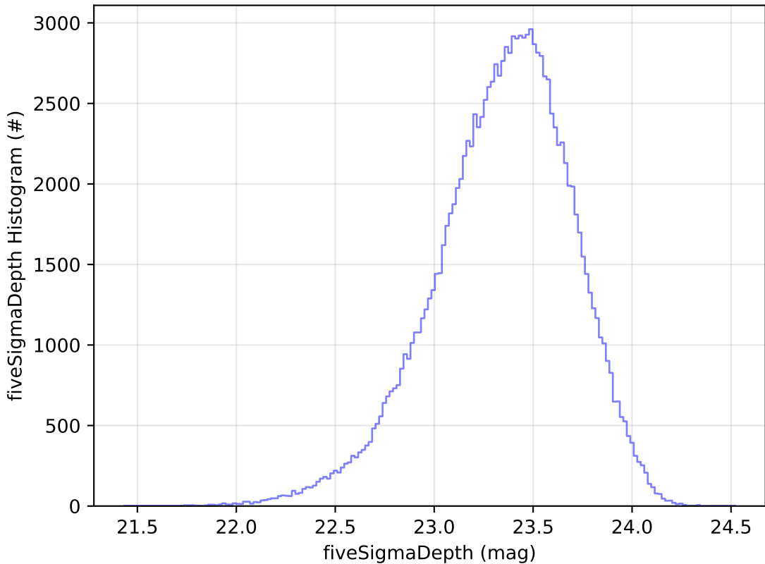
telescope_jerk_v3.5_10yrs All sky u band: fiveSigmaDepth Histogram
