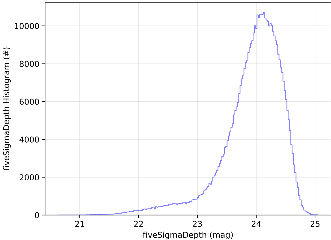
telescope_jerk_v3.5_10yrs All sky r band: fiveSigmaDepth Histogram
