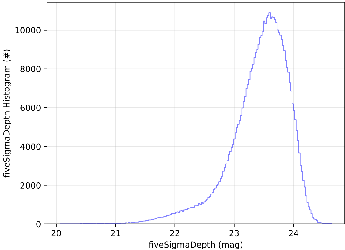
telescope_jerk_v3.5_10yrs All sky i band: fiveSigmaDepth Histogram
