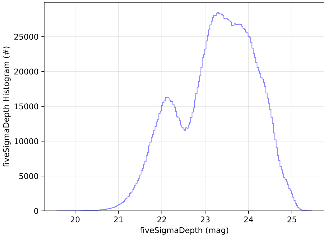
telescope_jerk_v3.5_10yrs All sky all bands: fiveSigmaDepth Histogram
