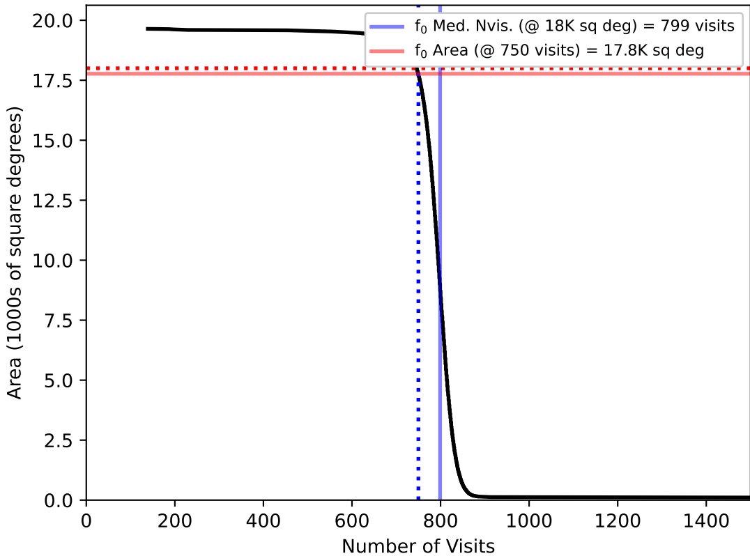
telescope_jerk_v3.5_10yrs WFD: f0
