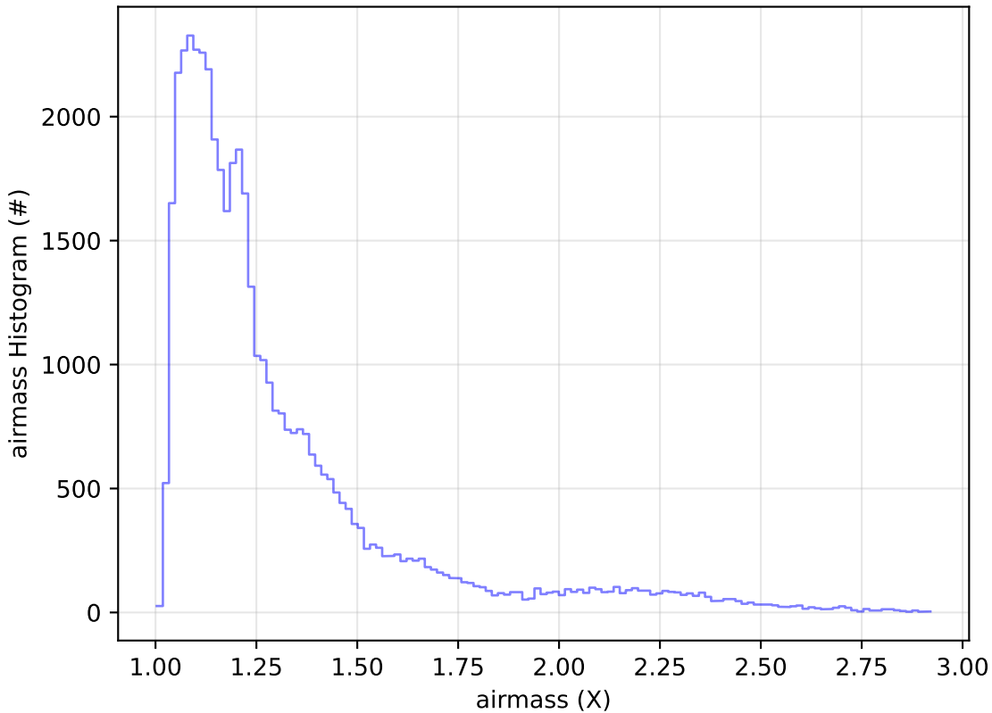
telescope_jerk_v3.5_10yrs Yr 1 z band: airmass Histogram
