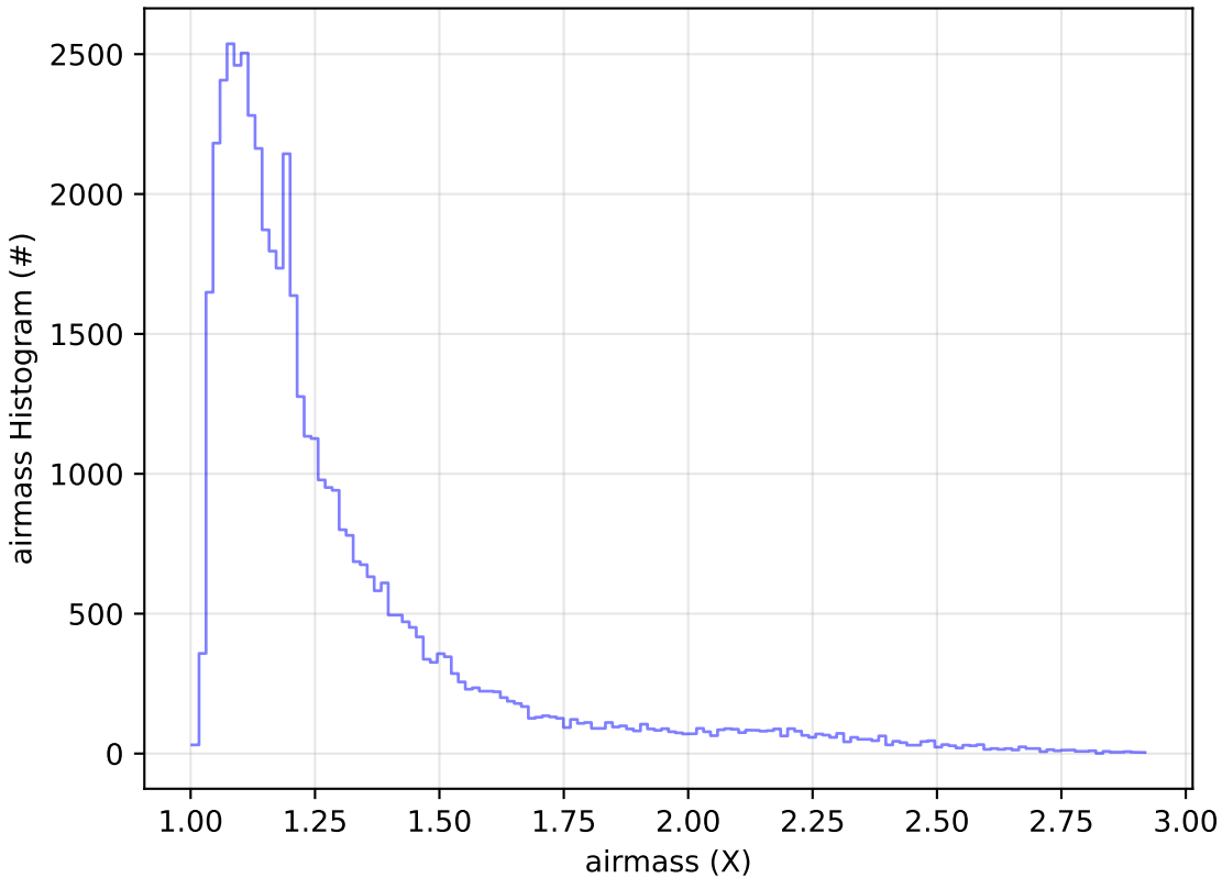
telescope_jerk_v3.5_10yrs Yr 1 r band: airmass Histogram
