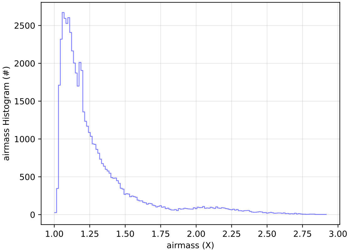
telescope_jerk_v3.5_10yrs Yr 1 i band: airmass Histogram
