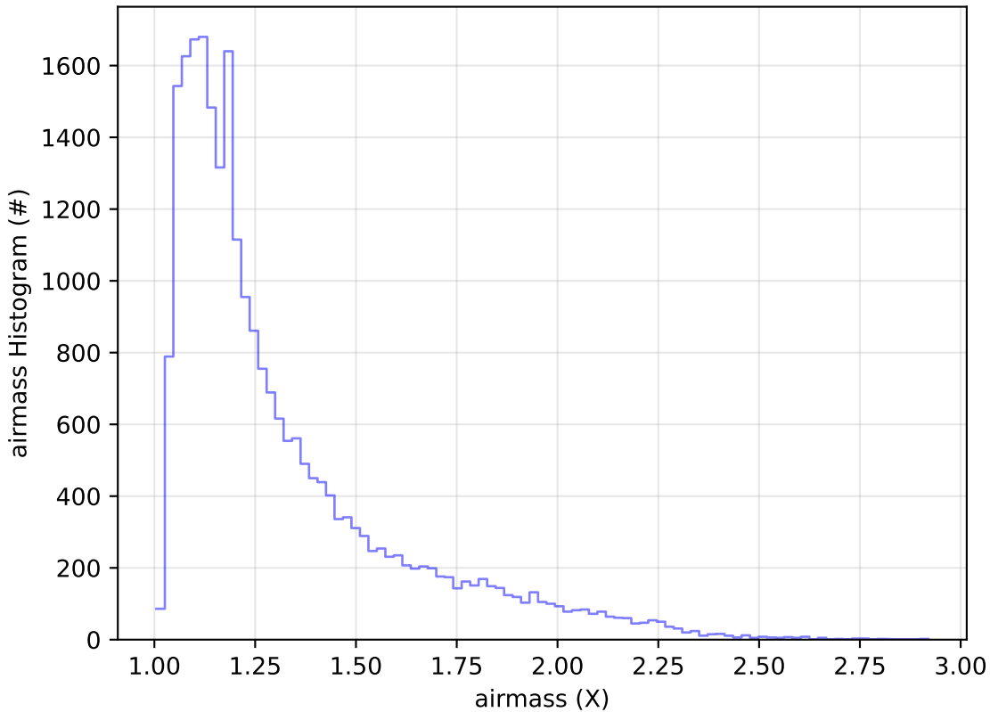
telescope_jerk_v3.5_10yrs Yr 1 g band: airmass Histogram
