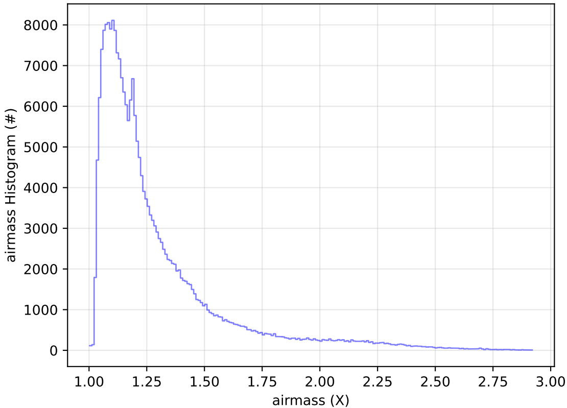
telescope_jerk_v3.5_10yrs Yr 1 all bands: airmass Histogram
