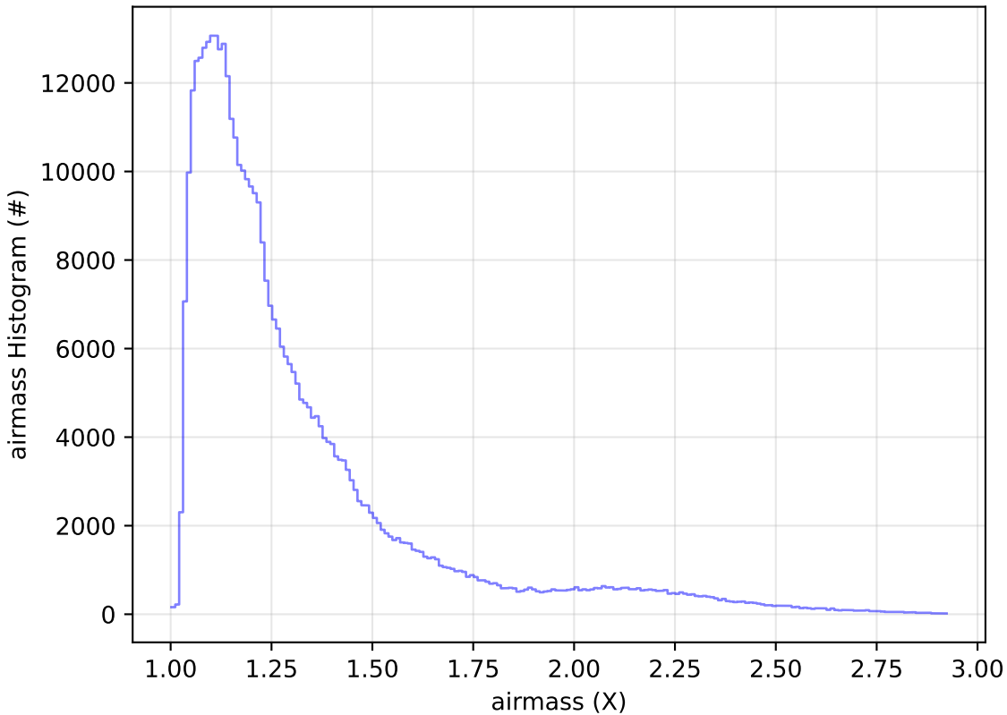
telescope_jerk_v3.5_10yrs WFD z band: airmass Histogram
