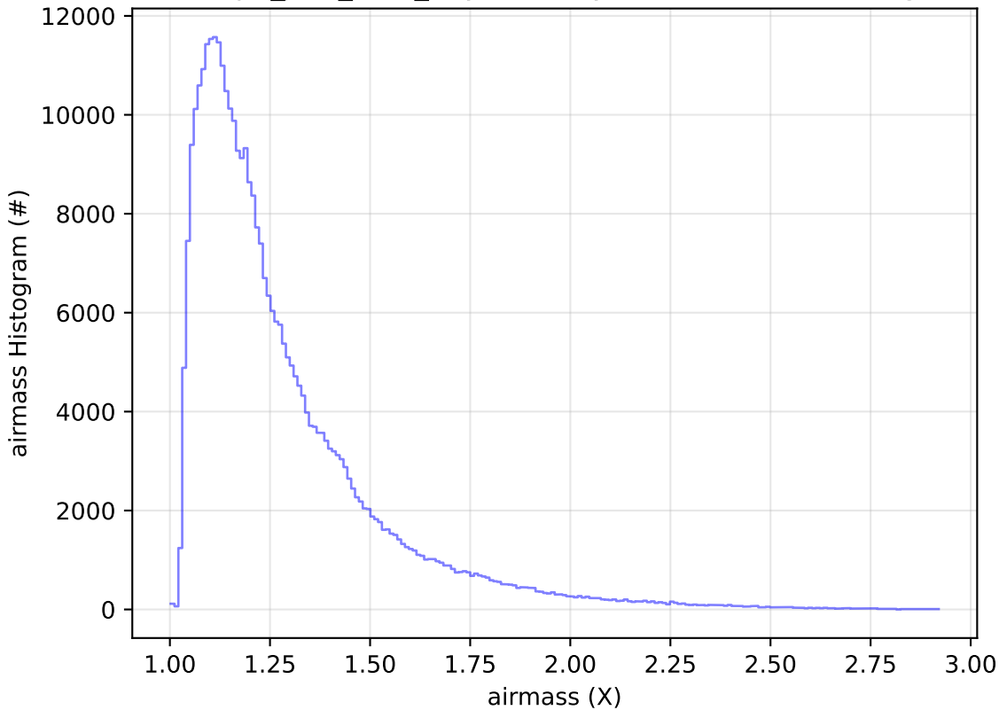
telescope_jerk_v3.5_10yrs WFD y band: airmass Histogram
