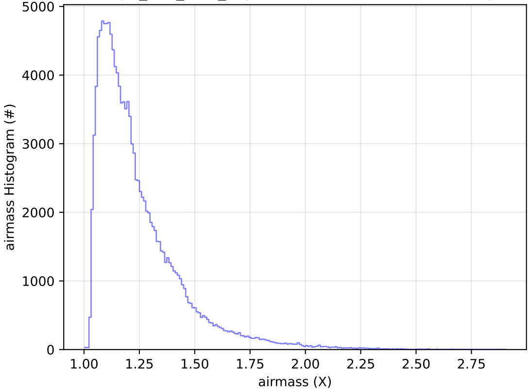
telescope_jerk_v3.5_10yrs WFD u band: airmass Histogram
