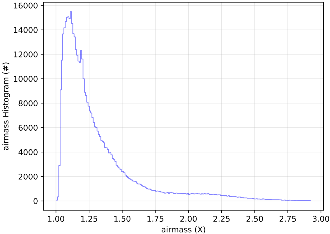
telescope_jerk_v3.5_10yrs WFD r band: airmass Histogram
